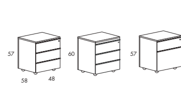
_CASSETTIERE SU RUOTE DRAWERS ON CASTORS / CAISSONS MOBILES
